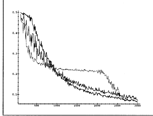
Figure 3. Experimental plots of generalization errors \epsilon_{\text{MDL}}(m) (most rapid initial decrease), \epsilon_{\text{CV}}(m) (intermediate initial decrease) and \epsilon_{\text{GRM}}(m) (least rapid initial decrease) versus sample size m for a target function of 100 alternating intervals and noise rate \eta = 0.20 . Each data point represents an average over 10 trials. Note that the “shelf” of \epsilon_{\text{MDL}} is approximately at the noise rate \eta = 0.20 , since MDL is coding all the noisy labels. Also, note by comparing the above plot to the plots in Figures 9 and 11 that the performance of MDL relative to the other two methods is degrading as the noise rate increases.
