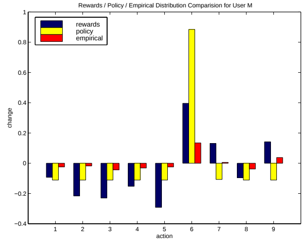
Figure 2: Rewards received, policy learned, and effect on actions for User M. For each of the nine RL actions, three quantities are represented. The blue bars (left) show the average reward given by User M for the corresponding action. The average reward given by User M across all actions has been subtracted off, so that “positive” bars indicate a relative preference for that action by User M, and “negative” bars indicate a relative objection to that action. The yellow bars (middle) show the policy (probability distribution) learned by Cobot for User M. The probability assigned to each action in the uniform distribution ( 1/9 ) has been subtracted off, so again the bars indicate relative preferences and objections of the learned policy. The red bars (right) show, for each action, the empirical frequency with which that action was taken by Cobot when User M was present, minus the empirical frequency with which that action was taken by Cobot over all time steps. Thus, these bars indicate the extent to which the presence of User M biases Cobot’s behavior towards M’s preferences. We see that (a) the policy learned by Cobot for User M aligns nicely with the preferences expressed by M through their training (comparison of left and middle bars), and (b) Cobot’s behavior shifts strongly towards the learned policy for User M whenever they are present (comparison of middle and right bars). The actions are presented here in the same order as in Table 1. To go beyond a qualitative visual analysis, we have defined a metric that measures the extent to which two rankings of actions agree, while taking into account the fact that some actions are numerically extremely close in the each ranking. While we do not have the space to provide details here, the agreement between the action rankings given by the rewards of User M and the policy learned for User M are in near-perfect agreement by this measure, as are the rankings given by the policy and the empirical distribution of rewards.
