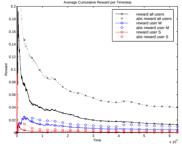
Figure 1: The average reward received by Cobot over time. The x-axis represents sequential Cobot-initiated RL actions for which it has received at least one reward or punishment event. The y-axis indicates the average cumulative reward received up to each such action. We examine both total reward (in which we sum the positive and negative values received), as well as absolute total reward (in which we ignore sign and simply count the total amount of feedback). We plot these quantities both over all users, and for two particular users we call Users M and S. In all cases, as time progresses, Cobot is receiving less feedback. This occurs despite the fact that Cobot is learning policies that coincide with the preferences of Users M and S, suggesting that this may not be a useful measure of performance.
